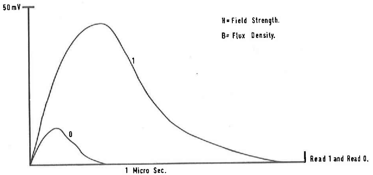
Fig o. Switching Response of Ferrite Core.
