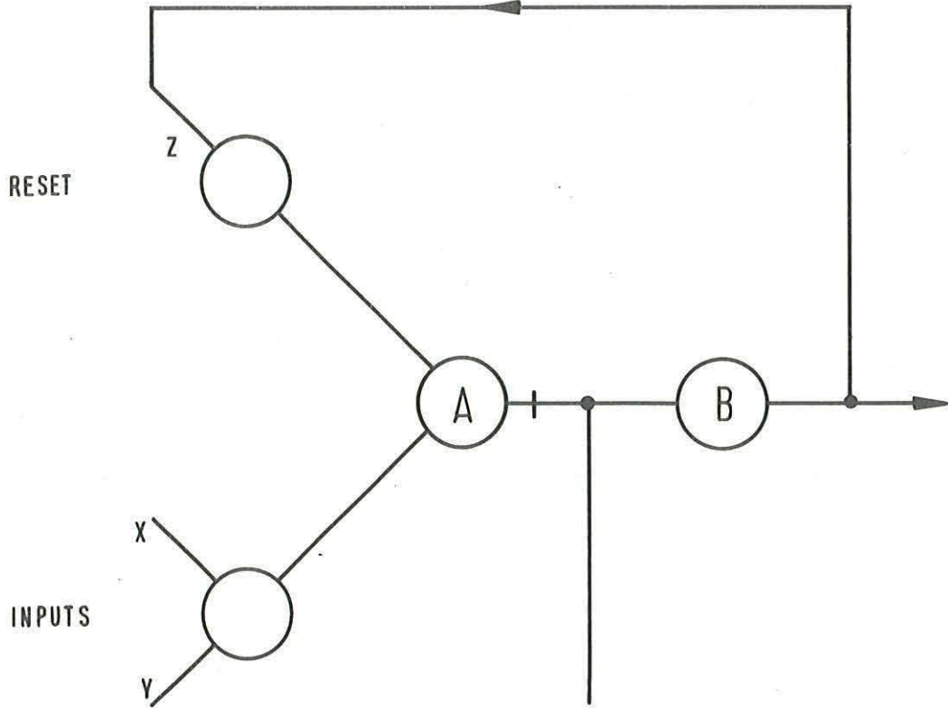
FIG. c. BISTABLE ELEMENT.
