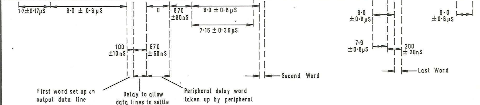
Fig. x. Block Output Timing
