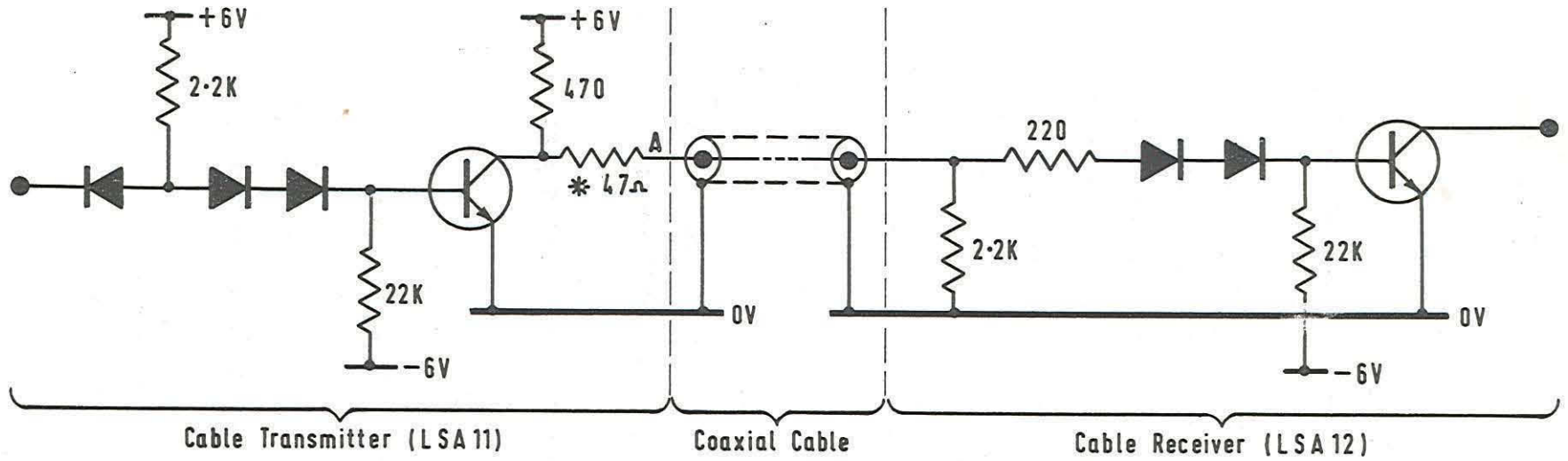
Fig. y. Cable Transmitter and Receiver (LSA 11 and 12)
